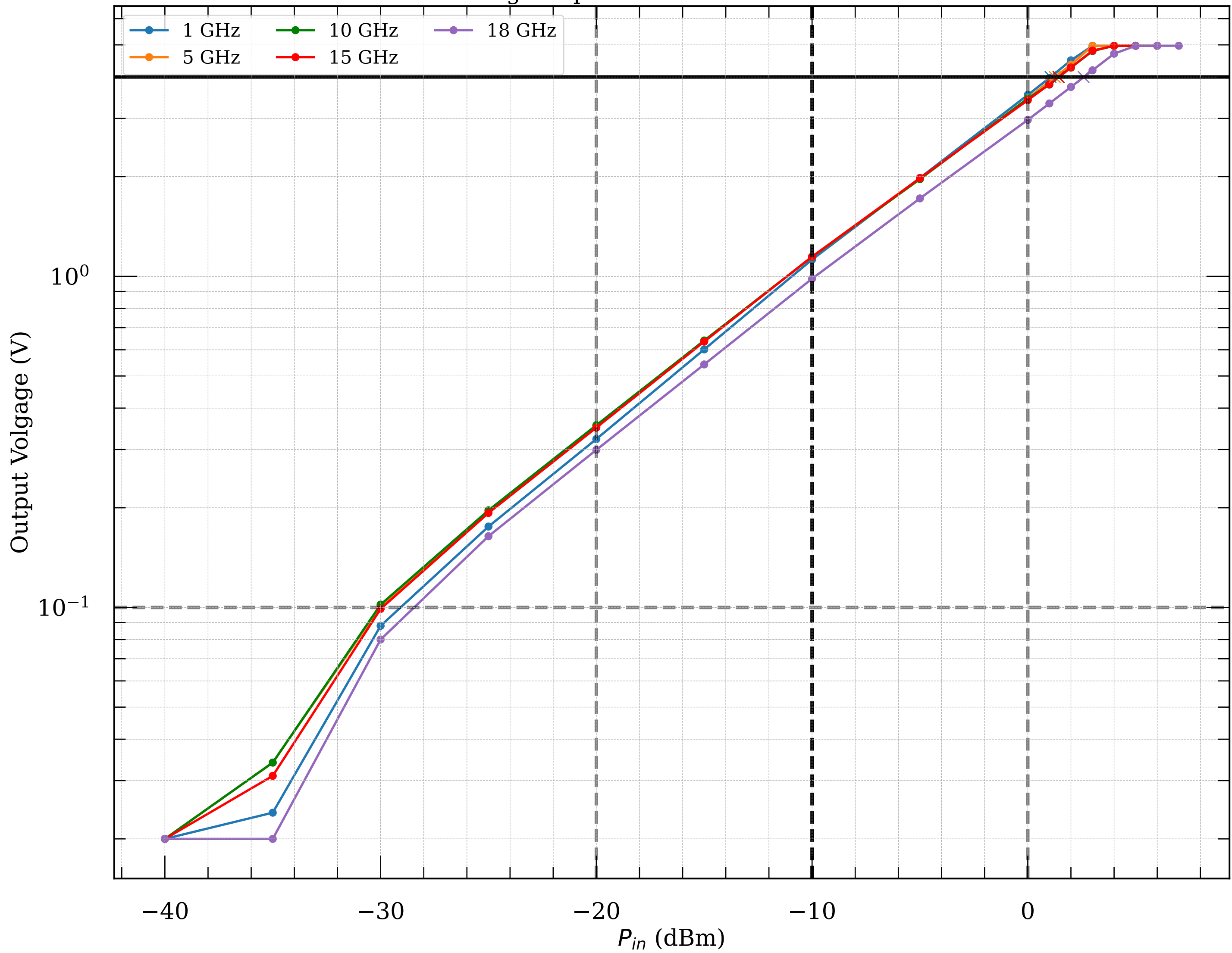
Measured voltage-to-power curve of detector module084v2
